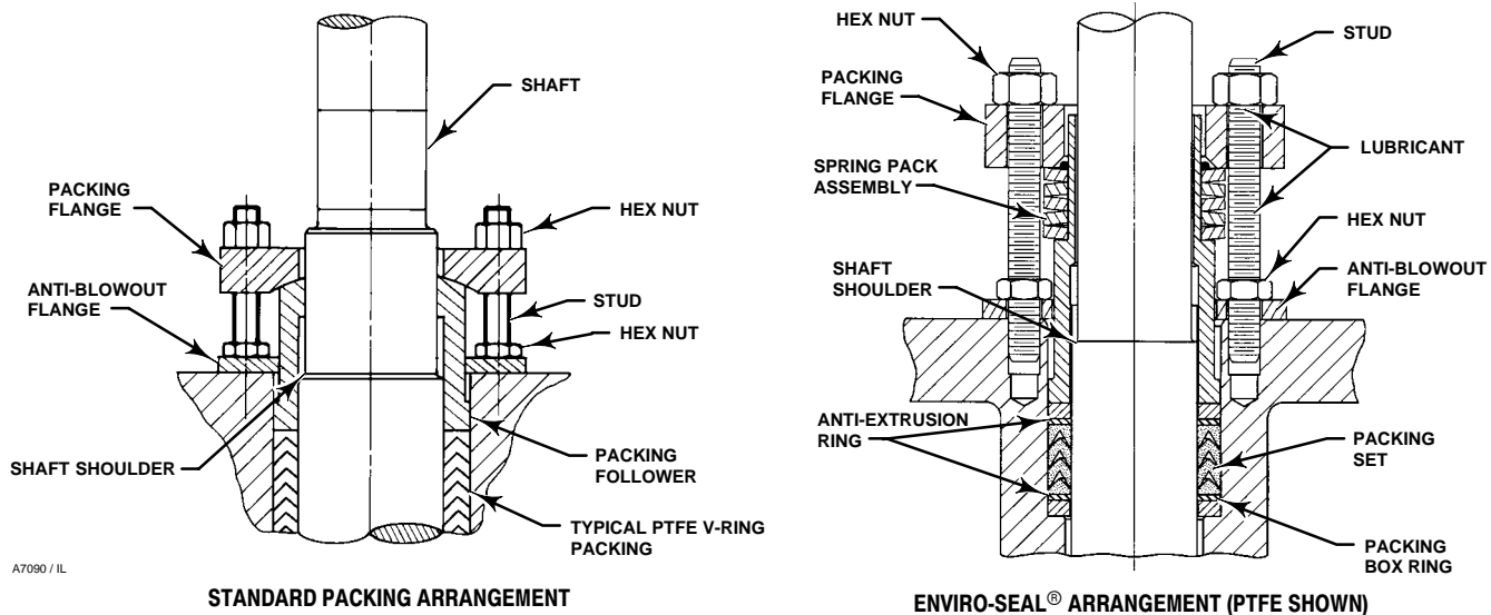
Figure 4. Blowout Protection
