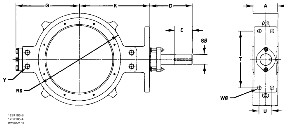
Figure 8. Dimensions and Weights, Wafer Style Valves, ANSI Class 300 (also see table 4)
